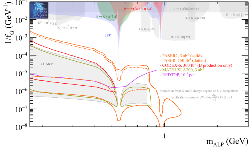
Figure 41: Current bounds (as coloured filled areas) and the prospects for PBC projects (solid lines) both on 5- (FASER) and 10-15 years (CODEX-b, MATHUSLA200, FASER2) timescale. The CHARM gray filled area has been computed by F. Kling, recasting the search for long-lived particles decaying to two photons performed at CHARM [193]. Other coloured filled areas are kindly provided by Mike Williams and revisited from Ref. [321]. The gray areas depend on UV completion and the results shown assume \approx [\log \Lambda_{\text{UV}}^2/m_t^2 \pm o(1)] \Rightarrow 1 . The CODEX-b curve has been obtained considering B-decays only, hence it is conservative. Both NA62 ++ and SHiP are sensitive to this benchmark case too, the curves are currently being compiled.
