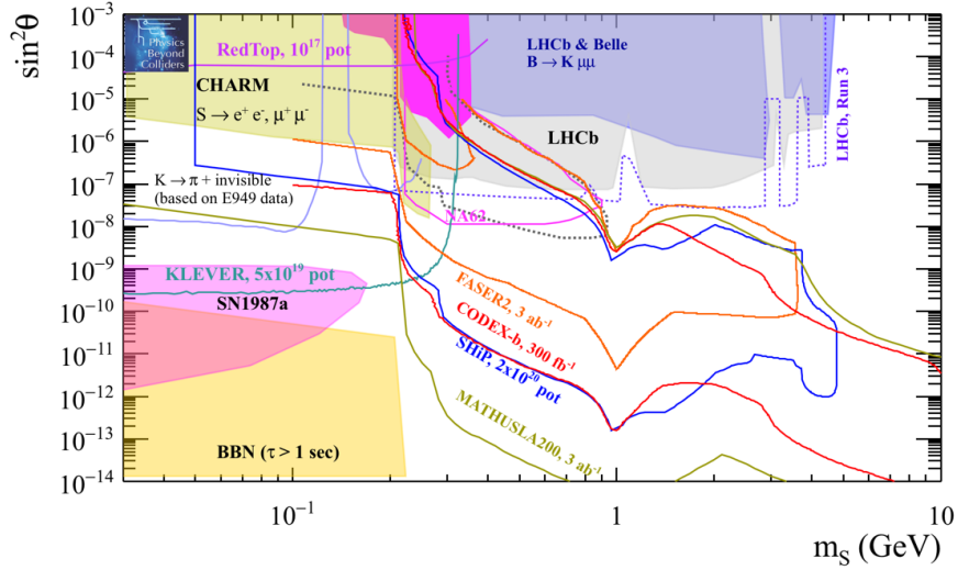
Figure 29: BC5: prospects in 10-15 years timescale for PBC projects for the dark scalar mixing with the Higgs in the plane mixing angle \sin^2 \theta versus dark scalar mass m_S under the hypothesis that both parameters \lambda and \mu are different from zero. The sensitivity curves have been obtained assuming BR(h \rightarrow SS) = 10^{-2} . The NA62 ++ and KLEVER curves correspond still to the case of \lambda = 0 , and, hence, should be considered conservative.
