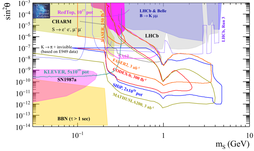
Figure 28: BC4: prospects in 10-15 years timescale for PBC projects for the Dark Scalar mixing with the Higgs in the plane mixing angle \sin^2 \theta versus dark scalar mass m_S .
