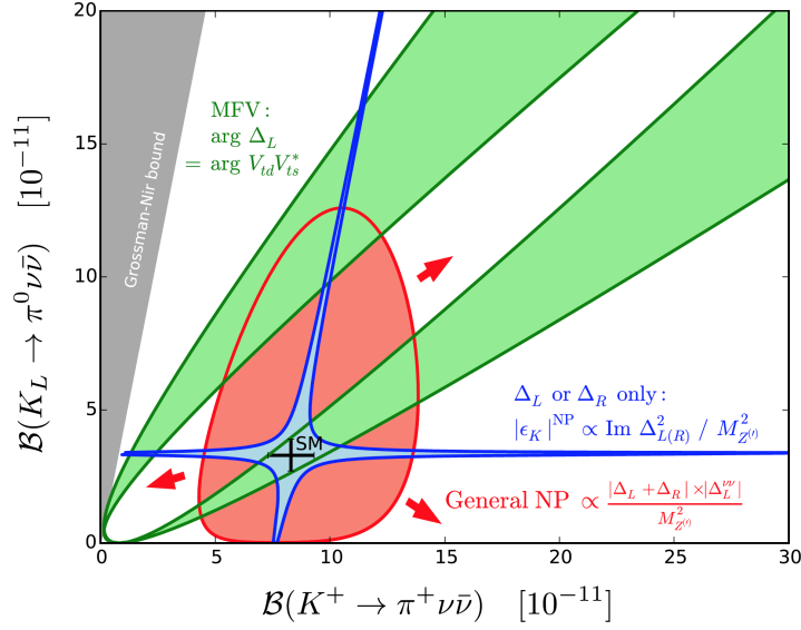
Figure 42: Scheme for BSM modifications of K \rightarrow \pi \nu \bar{\nu} BRs. Reproduced from Ref. [336].
