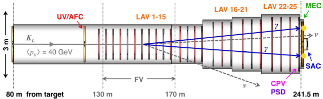
Figure 11: KLEVER experimental apparatus: upstream veto (UV), active final collimator (AFC), large-angle photon vetoes (LAV), main electromagnetic calorimeter (MEC), smallangle calorimeter (SAC), charged particle veto (CPV), pre-shower detector (PSD).
