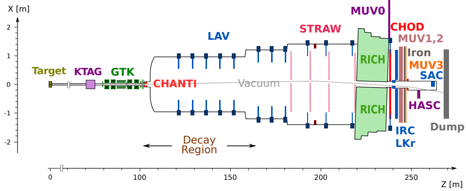
Figure 4: Layout of the NA62 experiment.
