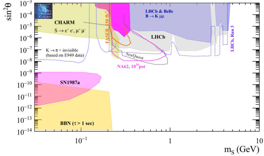
Figure 27: BC4: prospects in 5 years timescale for PBC projects for the dark scalar mixing with the Higgs in the plane mixing angle \sin^2 \theta versus dark scalar mass m_s . The two PBC projects that can provide results in 5-years timescale are NA62 ++ and FASER.
