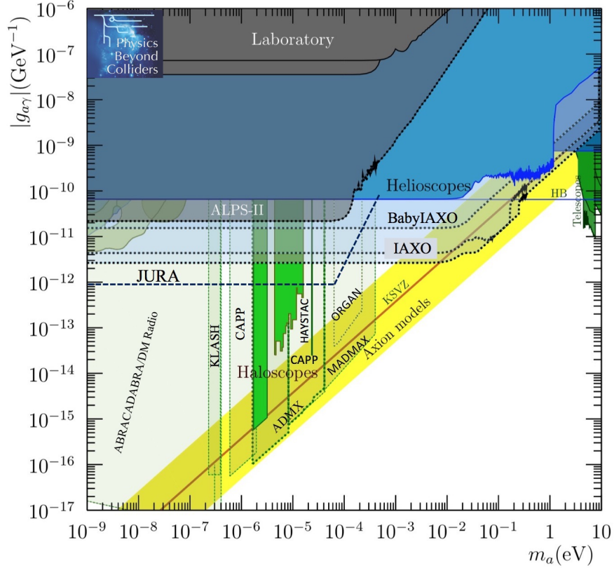
Figure 16: Physics reach of Baby-IAXO, IAXO and JURA compared with other experiments currently proposed and/or planned in the world. Revised from [39]. See text for details.
