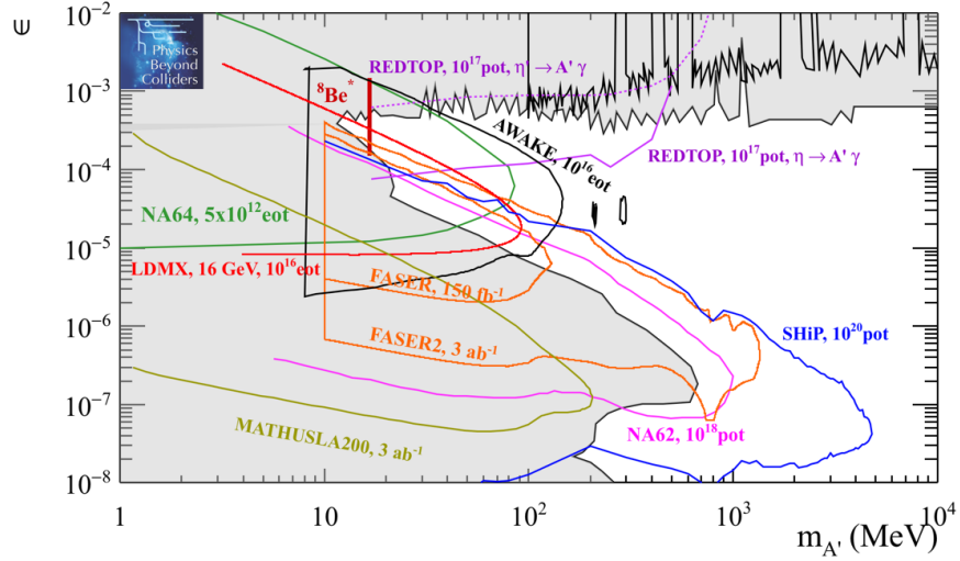
Figure 20: Future upper limits at 90 % CL for Dark Photon in visible decays in the plane mixing strength \epsilon versus mass m_{A'} for PBC projects with a timescale of \sim 10 -15 years. The vertical red line shows the allowed range of e - X couplings of a new gauge boson X coupled to electrons that could explain the ^8\text{Be} anomaly [72, 73].
