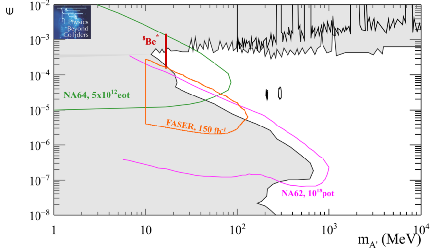
Figure 19: PBC projects with \sim 5 years timescale: upper limits at 90 % CL for Dark Photon in visible decays in the plane mixing strength \epsilon versus mass m_{A'} . The vertical red line shows the allowed range of e - X couplings of a new gauge boson X coupled to electrons that could explain the ^8\text{Be} anomaly [72, 73].
