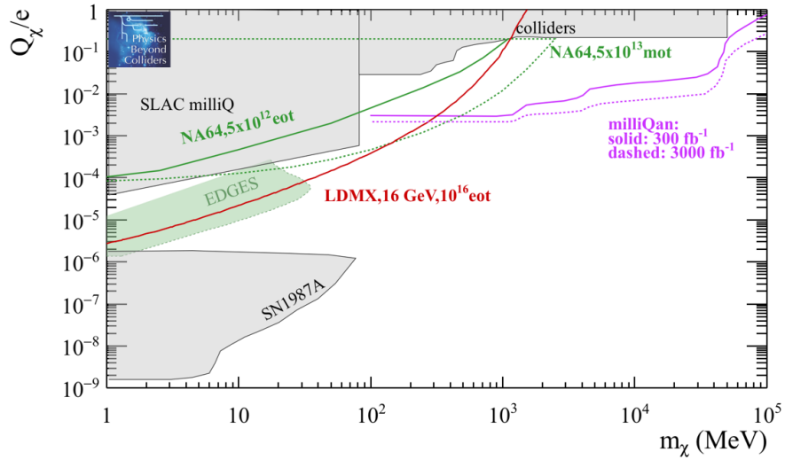
Figure 25: BC3: milli-charged particles. Current bounds (filled areas), experimental landscape and physics reach of PBC projects in 5 years time scale ( \text{NA64}^{++}(e) and \text{NA64}^{++}(\mu) ), and in 10-15 years time scale (LDMX @ eSPS).
