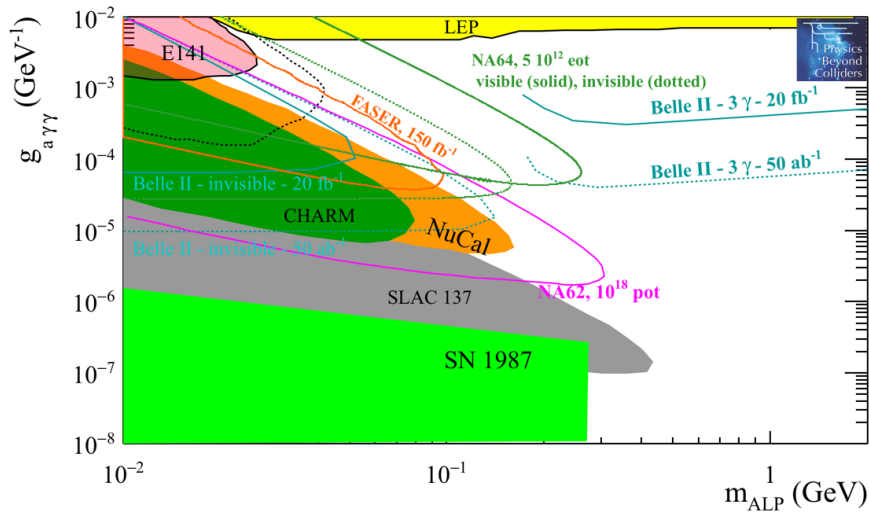
Figure 37: BC9: ALPs with photon coupling. Current bounds (filled areas) and prospects for PBC projects in 5 years timescale (solid lines) in the plane coupling g_{a\gamma\gamma} versus mass m_{ALP} . The results from a phenomenological study for Belle-II [300] is also shown.
