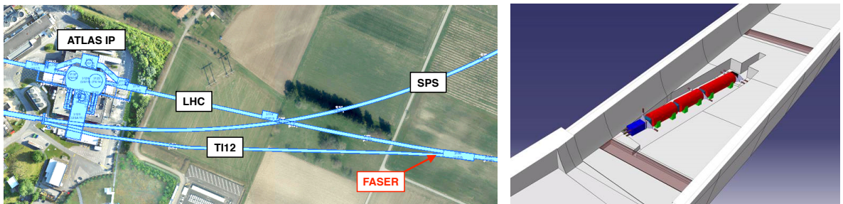
Figure 8: Left panel: The arrow points to FASER's location in service tunnel TI12, roughly 480 m east of the ATLAS IP. Credit: CERN Geographical Information System. Right panel: View of FASER in tunnel TI12. The trench lowers the floor by 45 cm at the front of FASER to allow FASER to be centered on the beam collision axis. Credit: CERN Site Management and Buildings Department.
