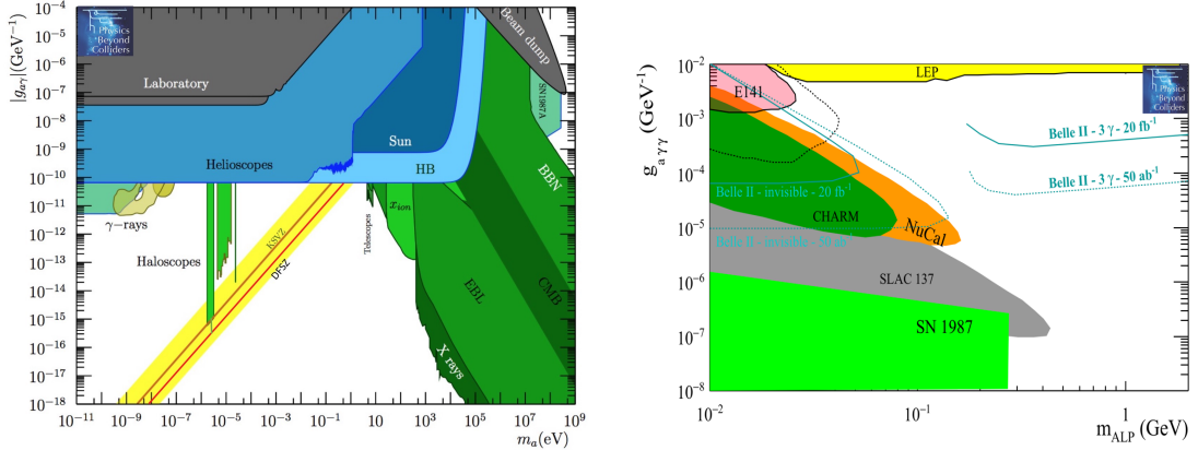
Figure 36: Left panel: current limits on axion with photon coupling in the plane coupling ( g_{a\gamma\gamma} ) versus mass ( m_a ). The right panel shows the zoom in the range of masses interesting for accelerator-based experiments (note the different units for the mass ranges in the two panels). In the left pane, current bounds are shown as filled coloured areas. A possible sensitivity from Belle-II from a phenomenological study [300] is also shown.
