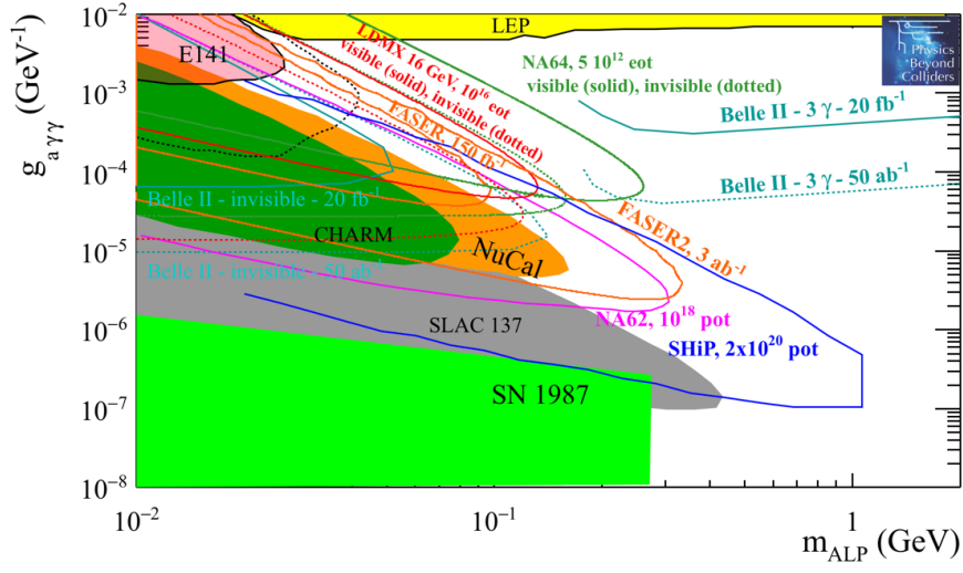
Figure 38: BC9: ALPs with photon coupling. Current bounds (filled areas) and prospects for PBC projects in 10-15 years timescale (solid lines) in the plane coupling g_{a\gamma\gamma} versus mass m_{ALP} . The results from a phenomenological study for Belle-II [300] is also shown.
