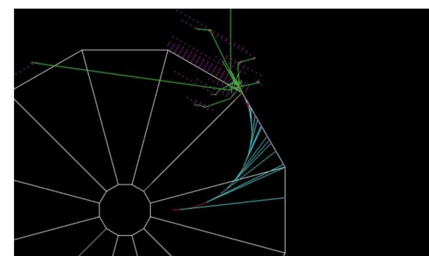
Figure 3. Representation of a 100 MeV electron (red track) traveling through the gas in a 0.6 T magnetic field. Several Cherenkov photons (cyan tracks) are generated and detected by the optical sensors surrounding the gas.
