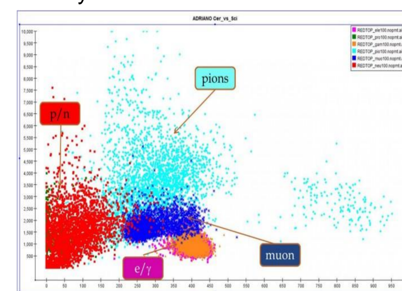
Figure 4. Particle identification from the comparison between the scintillation vs. Cherenkov signals in the ADRIANO calorimeter for simulated particles with E_{kin} = 100 MeV
