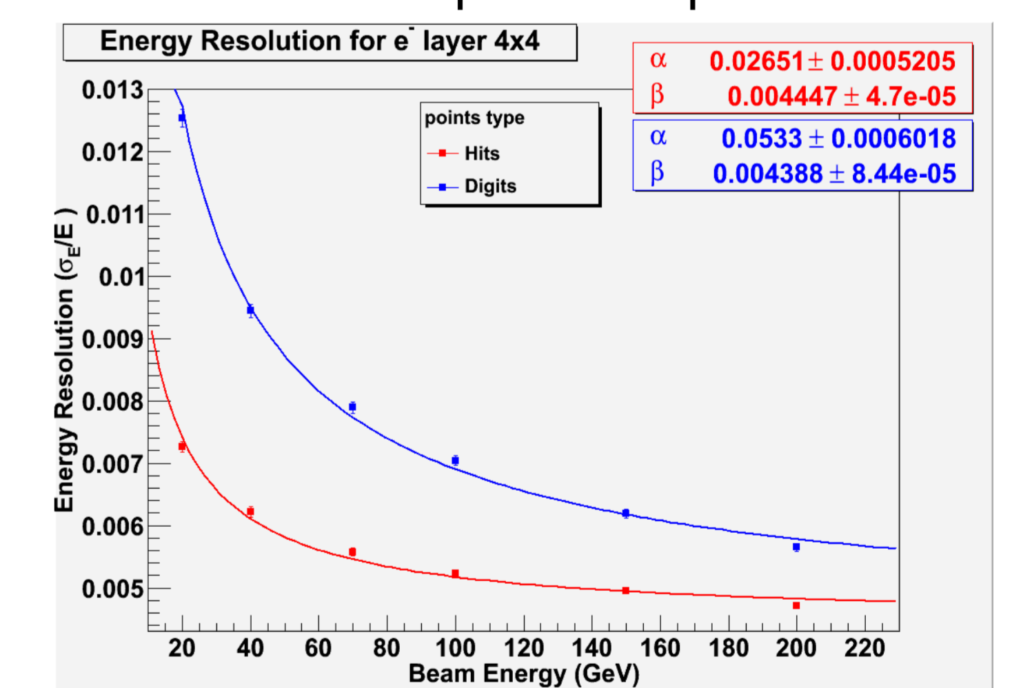
Figure 5. Energy resolution simulated with Ilroot.
