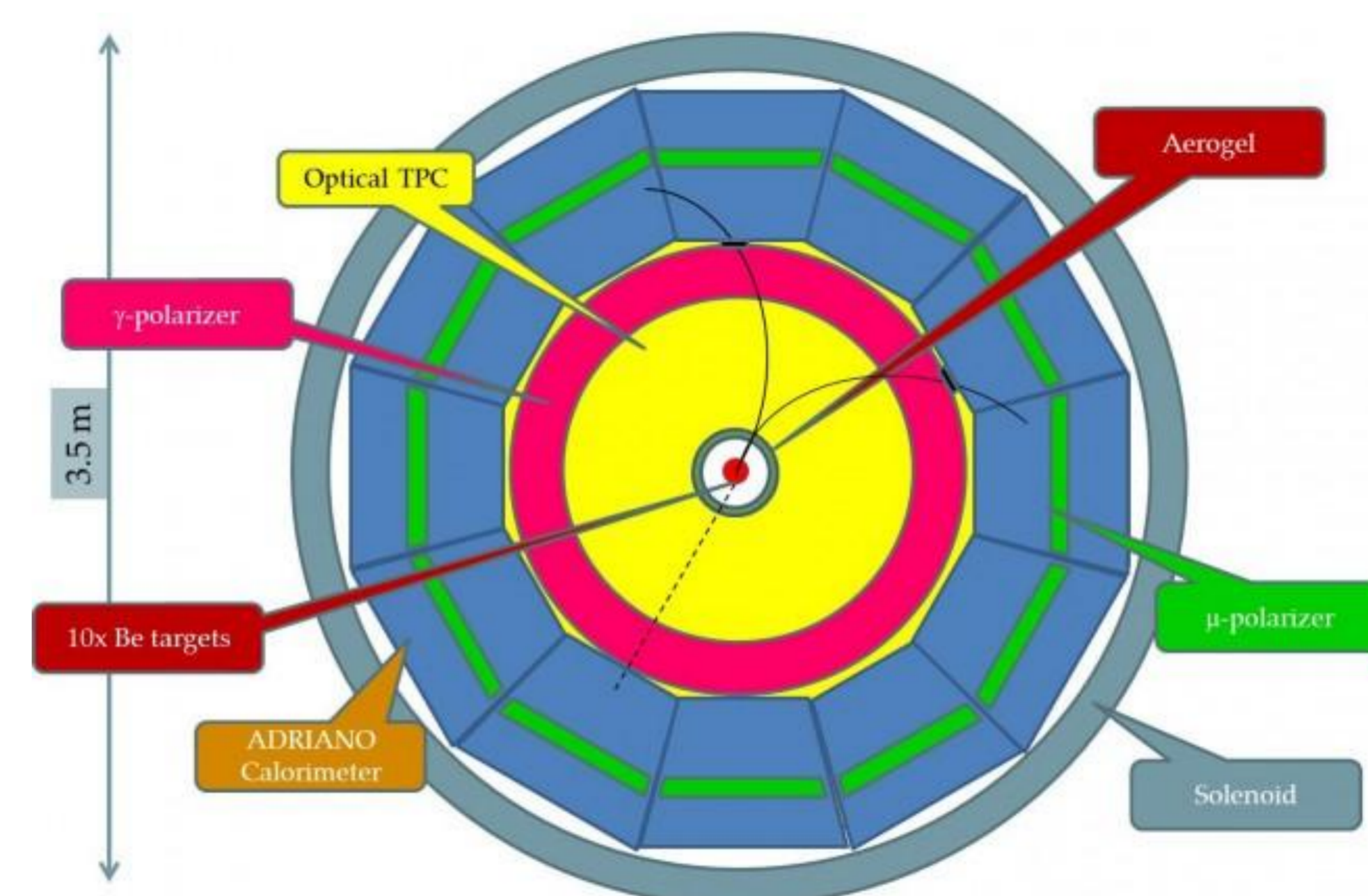
Figure 2. Schematics of the REDTOP detector.
