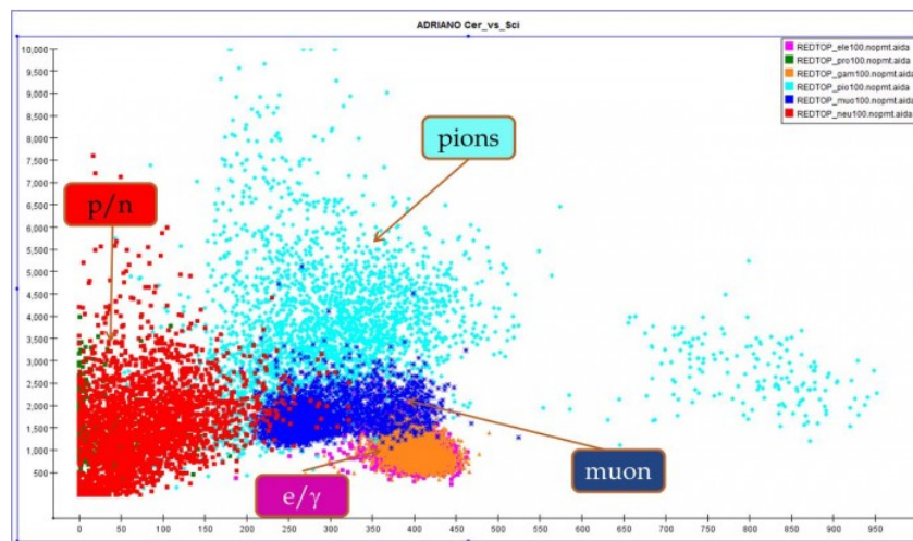
Figure 4: Particle identification from the comparison between the Scintillation vs. Cherenkov signals in the ADRIANO calorimeter for simulated particles with E_{kin} = 100 MeV.
